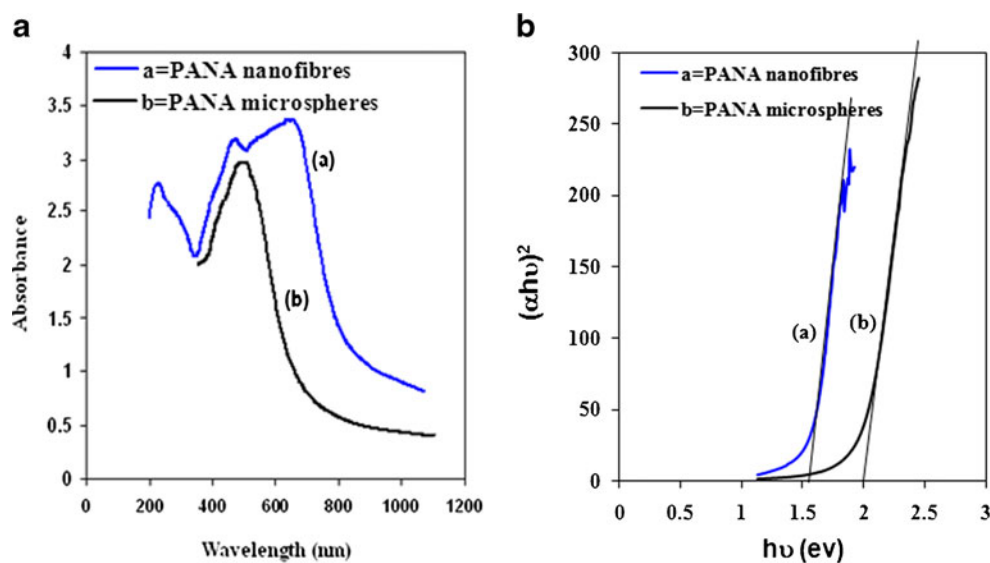
Fig. 8 a UV-vis spectra of PANA nanofibres at 0.1 M HCL/ \text{FeSO}_4 and microspheres at 0.1 M HCL in absence of \text{FeSO}_4 , b (\alpha h\nu)^2 vs. h\nu plot for bandgap estimation
