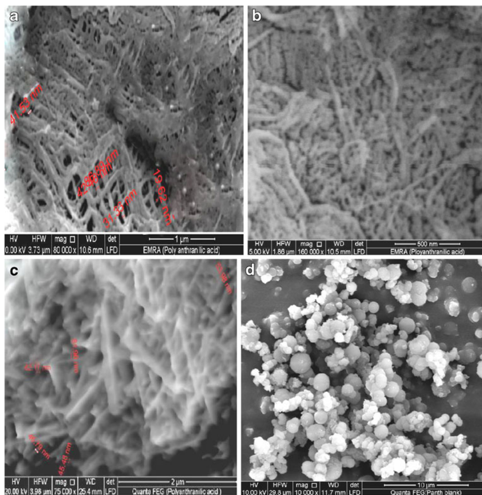
Fig. 1 SEM images of PANA. a nanofibres at 0.1 M HCL/FeSO 4 , b nanofibres at 0.5 M HCL/FeSO 4 , c nanorods at 0.1 M HCL/FeSO 4 (in dark) and d microspheres at 0.1 M HCL in absence of FeSO 4
